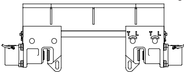
5' Caisson Beam with Model 100BH Caisson Clamps
